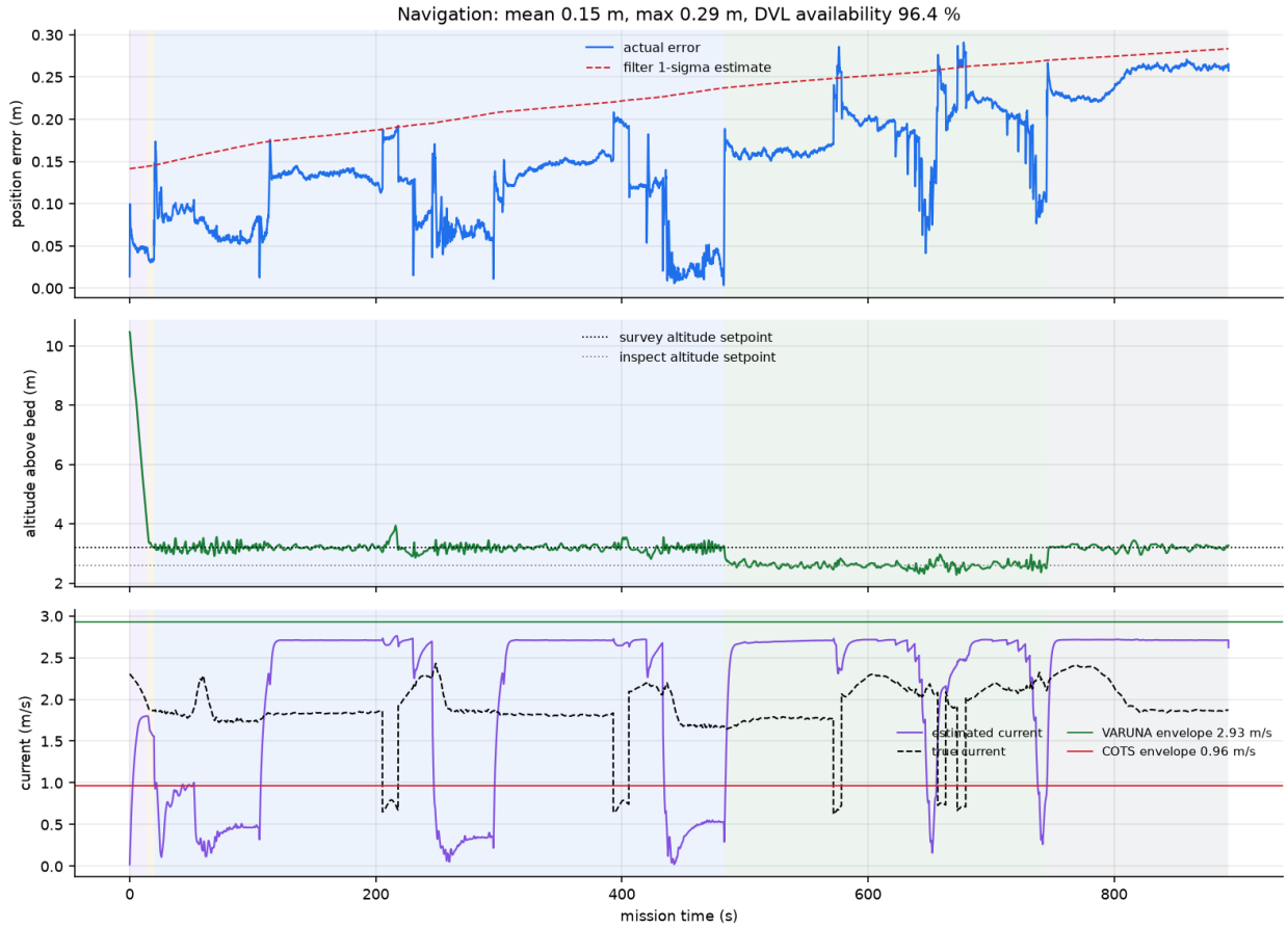
Figure 10: Navigation error against the filter’s own uncertainty estimate, altitude tracking, and estimated against true current with both vehicle envelopes marked.
