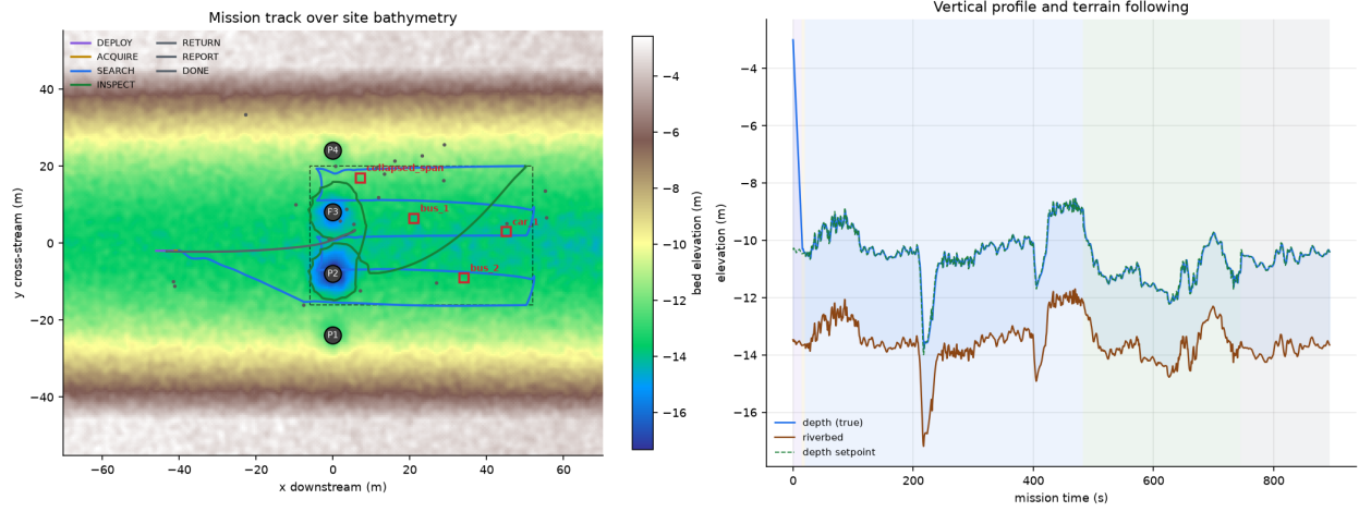
Figure 12: Mission track over site bathymetry, coloured by mission phase, and the vertical profile showing terrain following against the riverbed.
