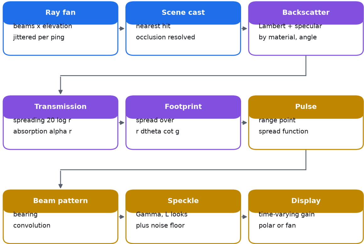
Figure 7: Sonar image formation. Every stage is a physical effect rather than a rendering convenience.
