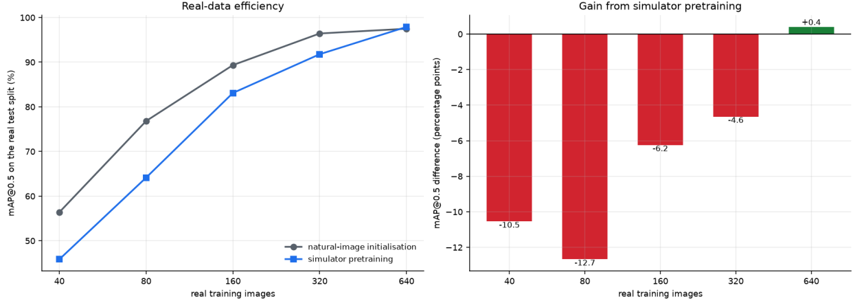
Figure 11: Real-data efficiency. Both arms are trained on the same real images and evaluated on the same real test split, differing only in initialisation. Simulator pretraining is worse at every size except the largest.
