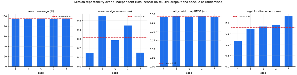
Figure 12: Per-seed results with the mean marked. The spread, not the best run, is the honest statement of what the system does.
