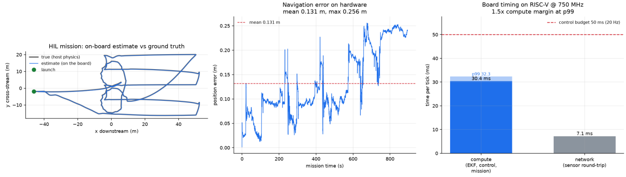
Figure 13: Full mission executed on the flight computer. Left: the on-board pose estimate against the host’s ground truth. Centre: navigation error over the run. Right: per-tick board timing, compute separated from the sensor round-trip, against the control budget.
