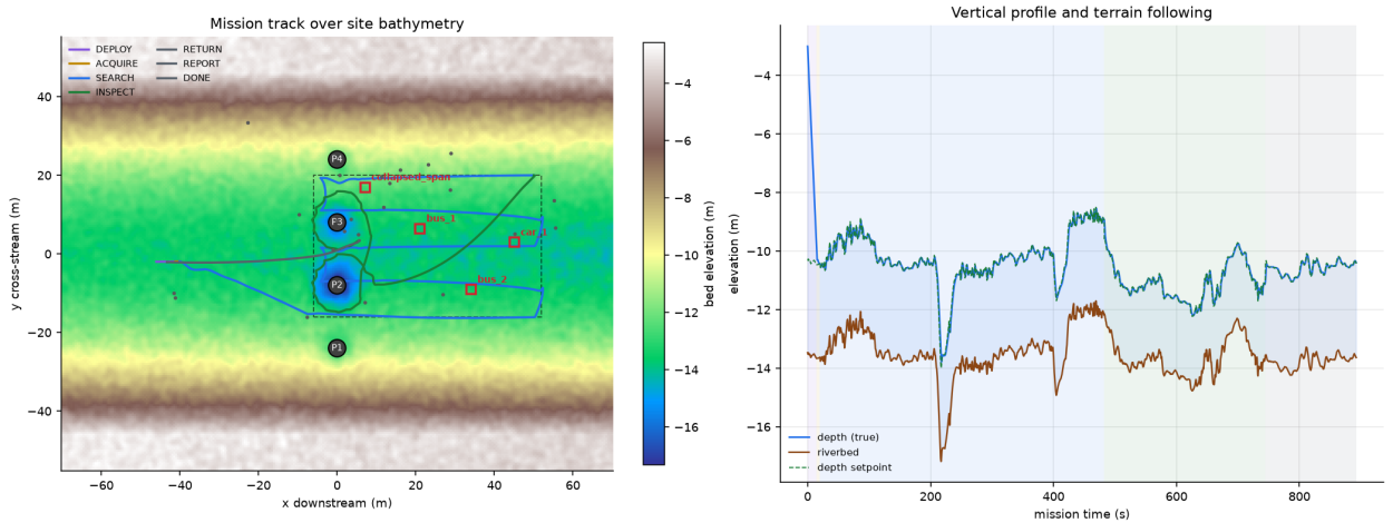
Figure 8: Mission track over site bathymetry, coloured by mission phase, and the vertical profile showing terrain following against the riverbed.
