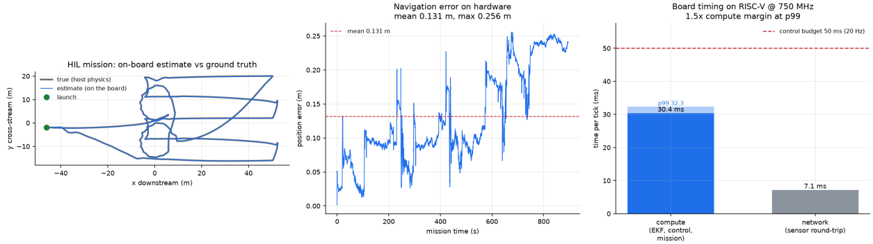
Figure 14: Full mission executed on the flight computer. Left: the on-board pose estimate against the host’s ground truth. Centre: navigation error over the run. Right: per-tick board timing, compute separated from the sensor round-trip, against the control budget.
