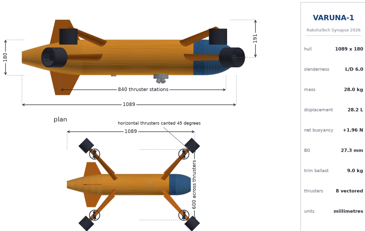
Figure 3: Principal dimensions. The hull form, the thruster stations and the 45° cant all come from the parameters the dynamics model uses.
