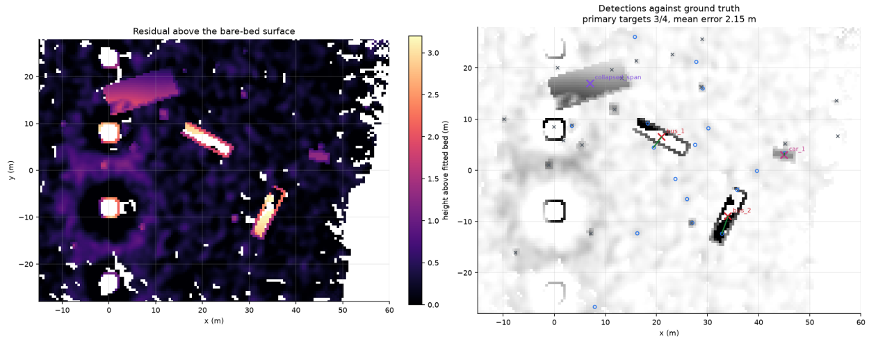
Figure 8: Left: height above the fitted bare bed surface. Right: detections against ground truth, with green lines joining each matched pair.
