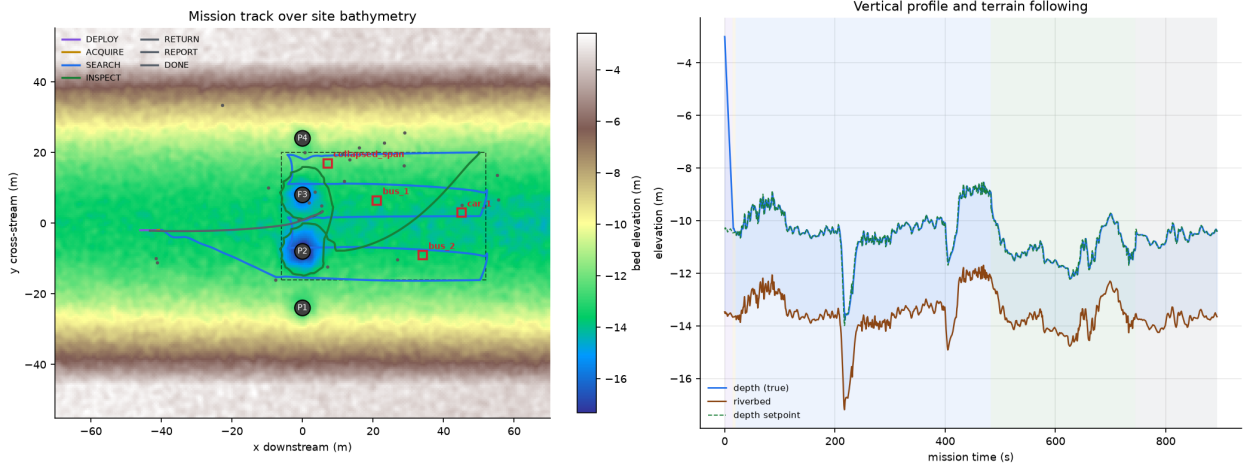
Figure 9: Mission track over site bathymetry, coloured by mission phase, and the vertical profile showing terrain following against the riverbed.
