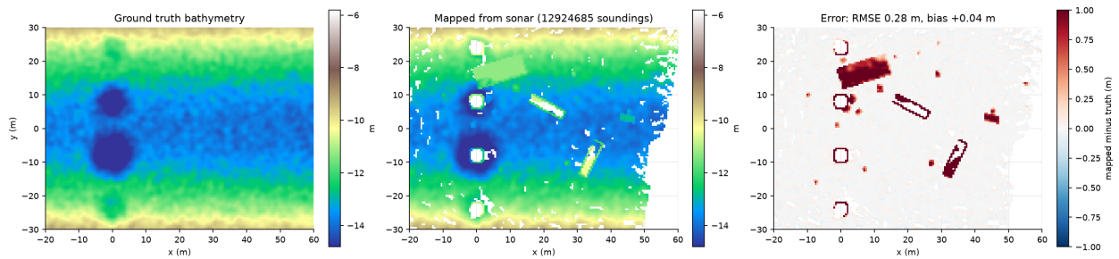
Figure 11: Ground truth bathymetry, the map built from simulated sonar during the mission, and the difference. The residual is near zero over open bed; the remaining structure is the submerged objects, which stand above the bare bed and are the subject of Section 7.
