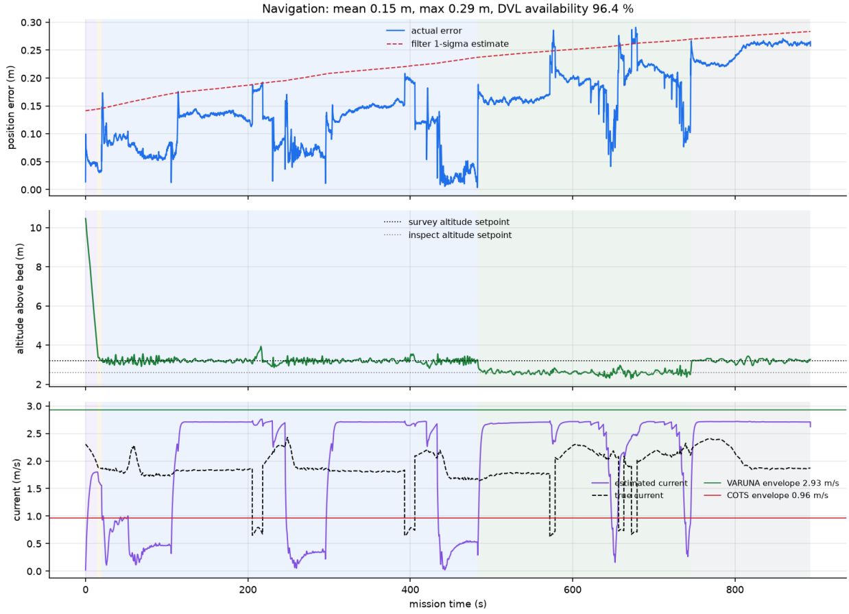
Figure 13: Navigation error against the filter’s own uncertainty estimate, altitude tracking, and estimated against true current with both vehicle envelopes marked.
