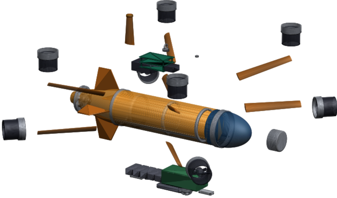
Figure 6: The same vehicle as a parts breakdown. Every line of the mass budget is a solid in the model, 52 parts in all: the eight thruster pods with their ducts and pylons, the ring frames, the nose dome, the fins, the acoustic window, the internal stack and the trim ballast. The budget in Table 2 is therefore a property of the geometry rather than a list kept alongside it, which is what allows the hull size, the ballast mass and the ballast station to be solved rather than chosen.
