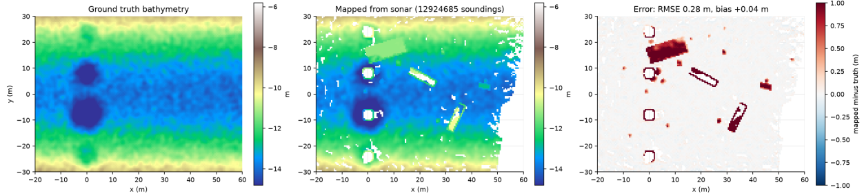
Figure 14: Ground truth bathymetry, the map built from simulated sonar during the mission, and the difference. The residual is near zero over open bed; the remaining structure is the submerged objects, which stand above the bare bed and are the subject of Section 7.
