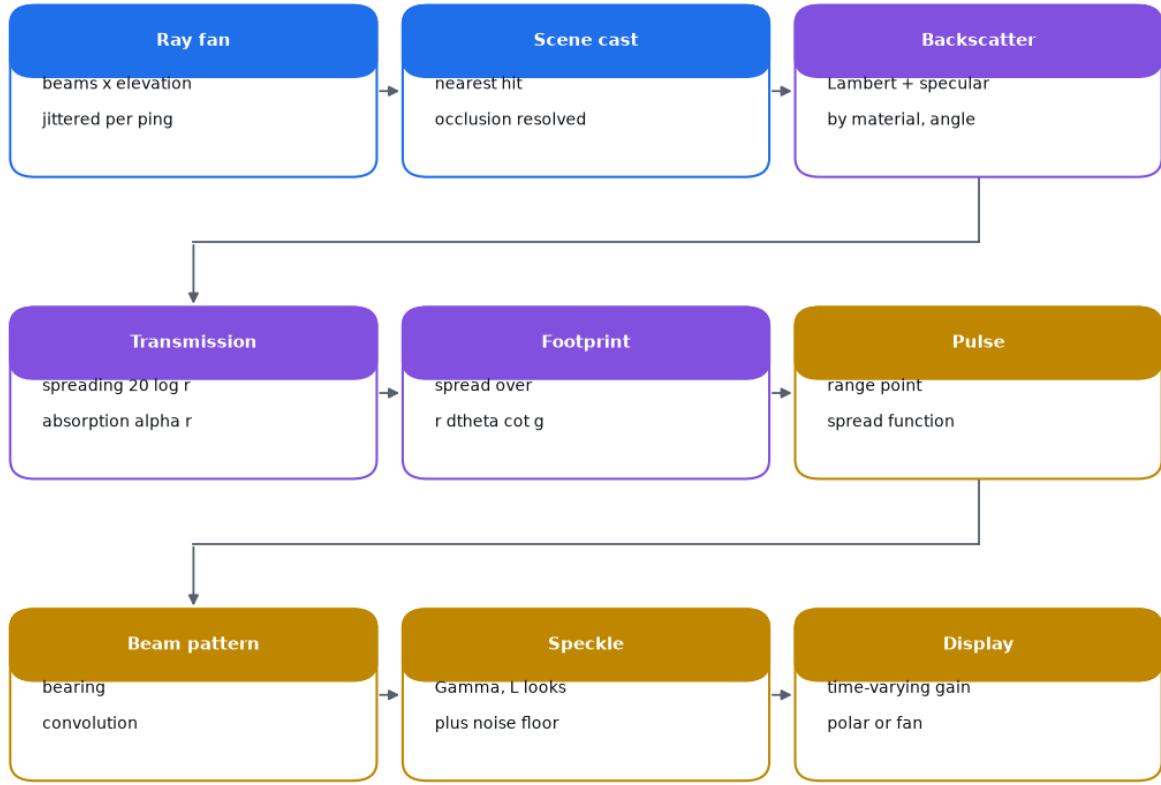
Figure 6: Sonar image formation. Every stage is a physical effect rather than a rendering convenience.
