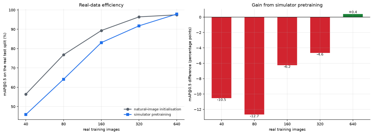
Figure 14: Real-data efficiency. Both arms are trained on the same real images and evaluated on the same real test split, differing only in initialisation. Simulator pretraining is worse at every size except the largest.
