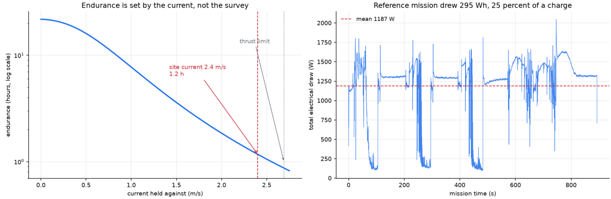
Figure 16: Left: endurance holding station, against the current being fought. Right: the electrical draw of the reference mission, integrated from the logged thruster forces. The low sections are downstream legs, the high ones are upstream legs and station keeping.
