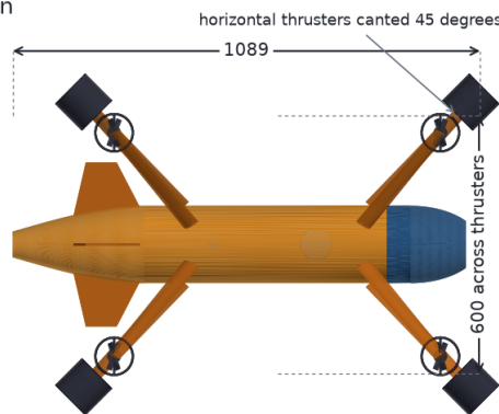
Figure 3: Principal dimensions. The hull form, the thruster stations and the 45° cant all come from the parameters the dynamics model uses.
