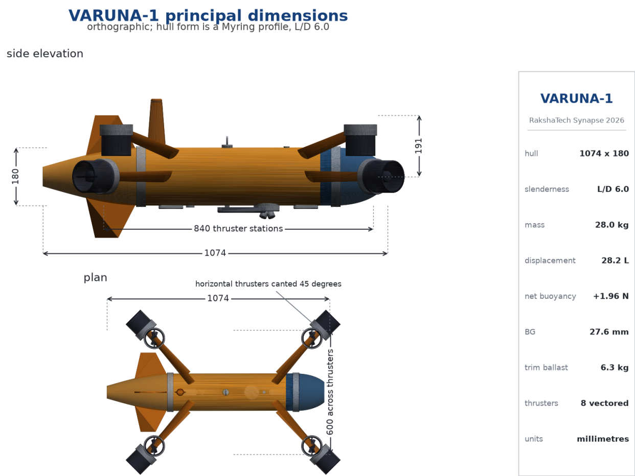
Figure 4: Principal dimensions. The hull form, the thruster stations and the 45° cant all come from the parameters the dynamics model uses.
