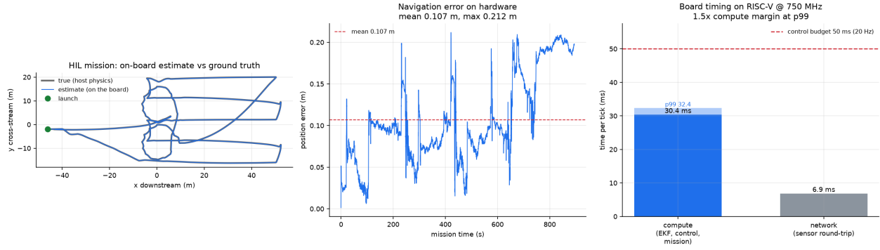
Figure 15: Full mission executed on the flight computer. Left: the on-board pose estimate against the host’s ground truth. Centre: navigation error over the run. Right: per-tick board timing, compute separated from the sensor round-trip, against the control budget.
