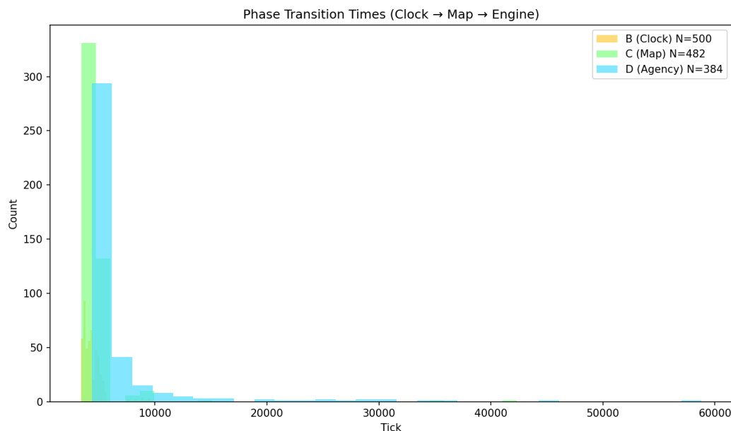
Figure 1. Phase transition time distributions from the 1D Monte Carlo study ( N = 500 ). Three overlapping histograms show when each phase transition occurred across all runs. The distributions are clearly ordered — Clock (B, amber) is leftmost, Map (C, green) next, Agency (D, cyan) rightmost.
