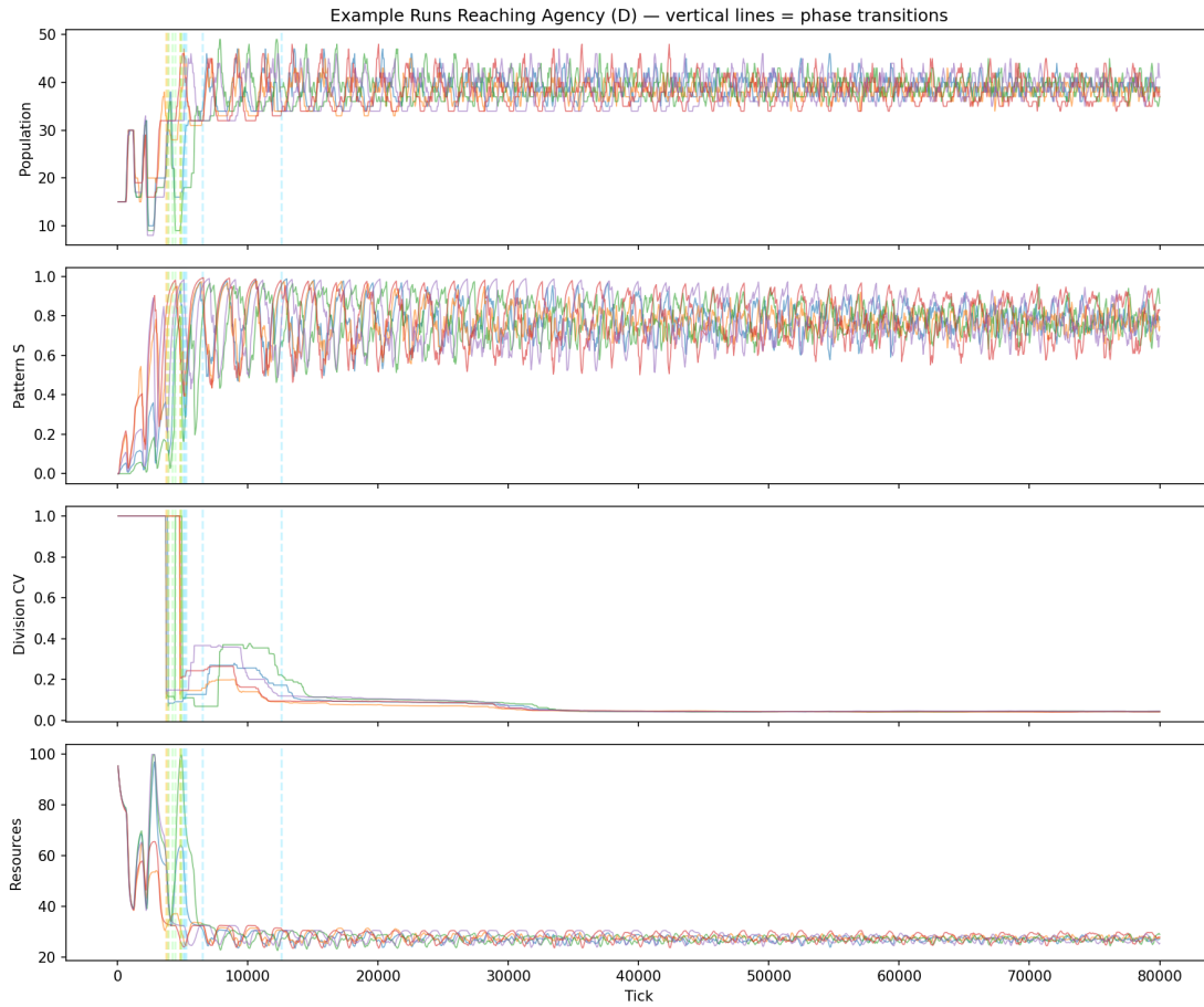
Figure 3. Example time series traces from five runs reaching Phase D. Four panels show population, pattern stability S , division CV , and resource levels across 80,000 ticks. Vertical dashed lines mark phase transitions (amber = B, green = C, cyan = D). The visual signature of the mandatory ordering is clear: CV crashes first, then S rises, then population stabilizes.
