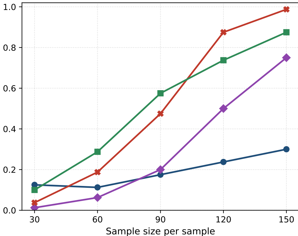
Power: A=(NORM, STR, LYM) vs B=(TUM, STR, LYM)
