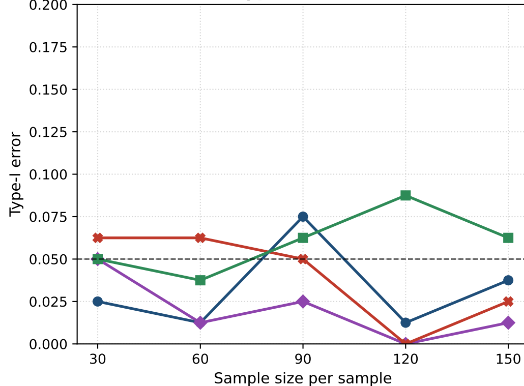
Type-I: A vs A
