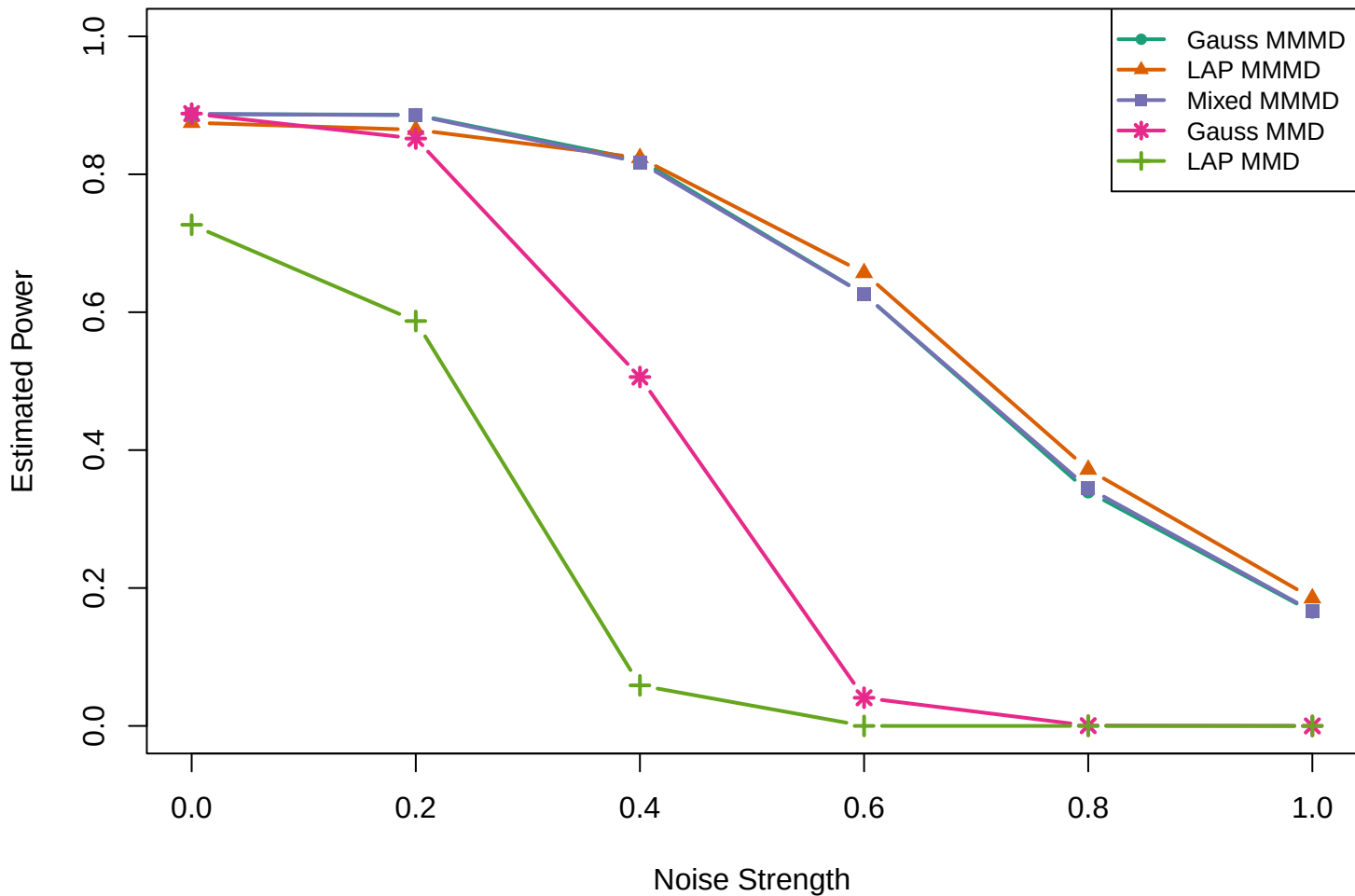
MNIST Additive Noise: {1,2,3} vs {1,2,8}
