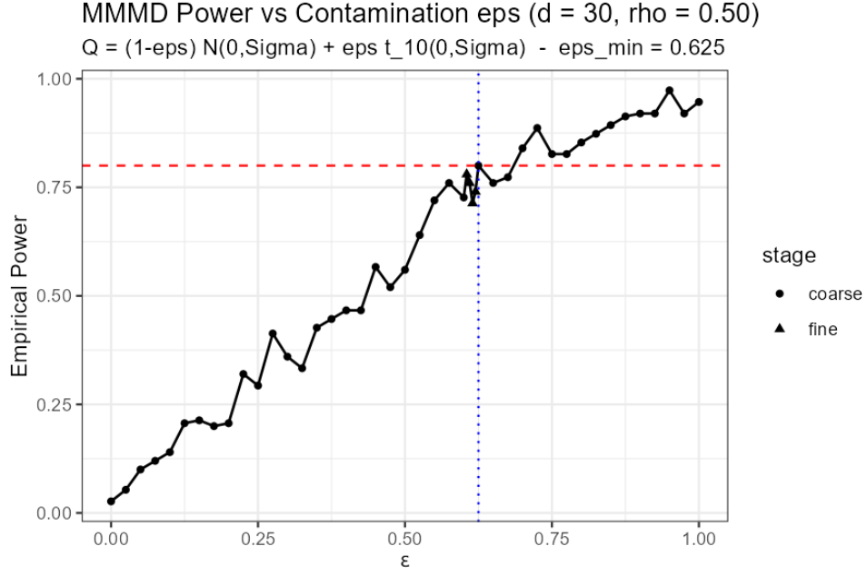
Figure 9: \epsilon -contamination sensitivity. P = \mathcal{N}(0, \Sigma) , Q = (1 - \epsilon)\mathcal{N}(0, \Sigma) + \epsilon \cdot t_{10}(0, \Sigma) . GEXP kernel, r = 5 , n = 100 . Power reaches 0.80 at \epsilon = 0.625 .
