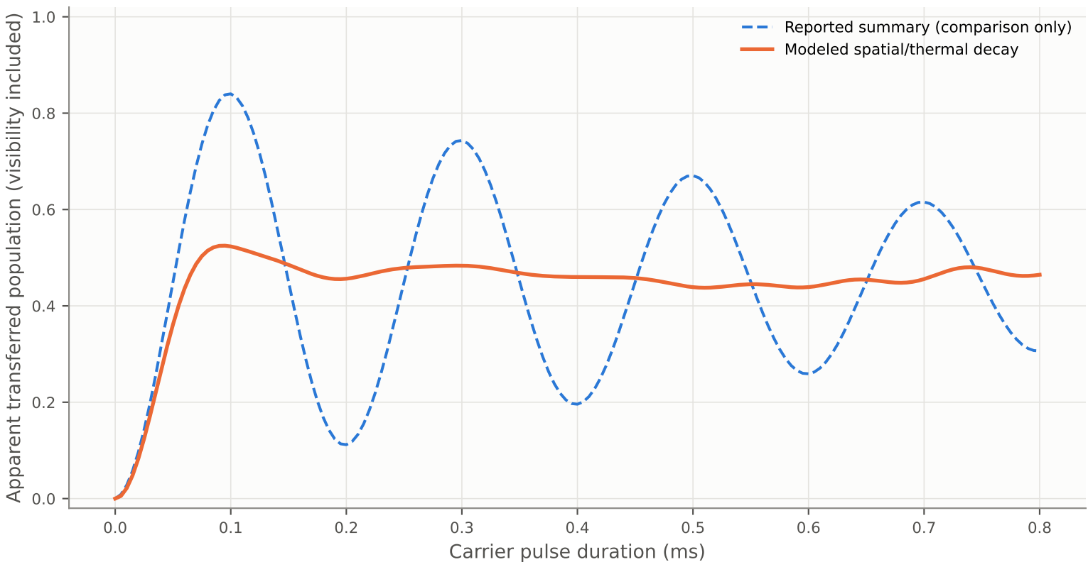
Modeled carrier decay; RMS Rabi 5 kHz Initial-curvature intensity calibration; no fitted damping
