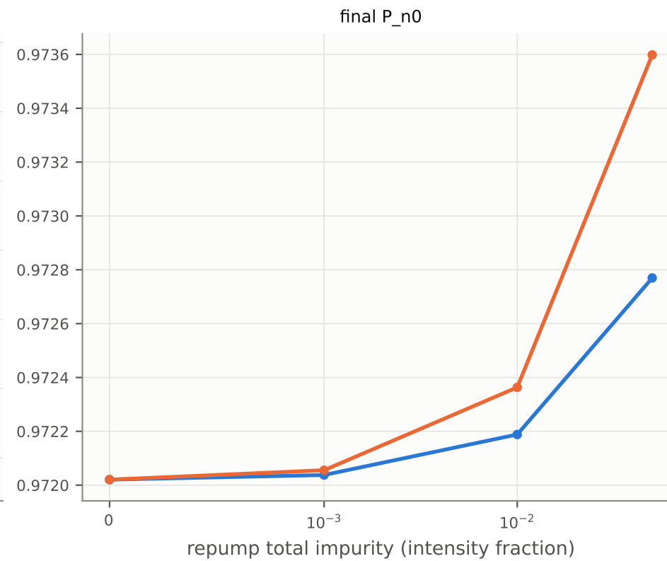
Repump polarization impurity: pi vs sigma- at equal total impurity (continuous, 5 ms)
