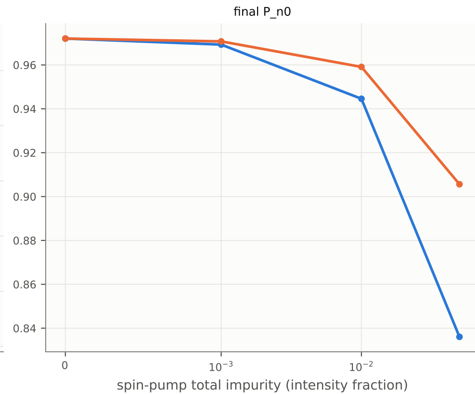
Spin-pump polarization impurity: pi vs sigma- at equal total impurity (continuous, 5 ms)
