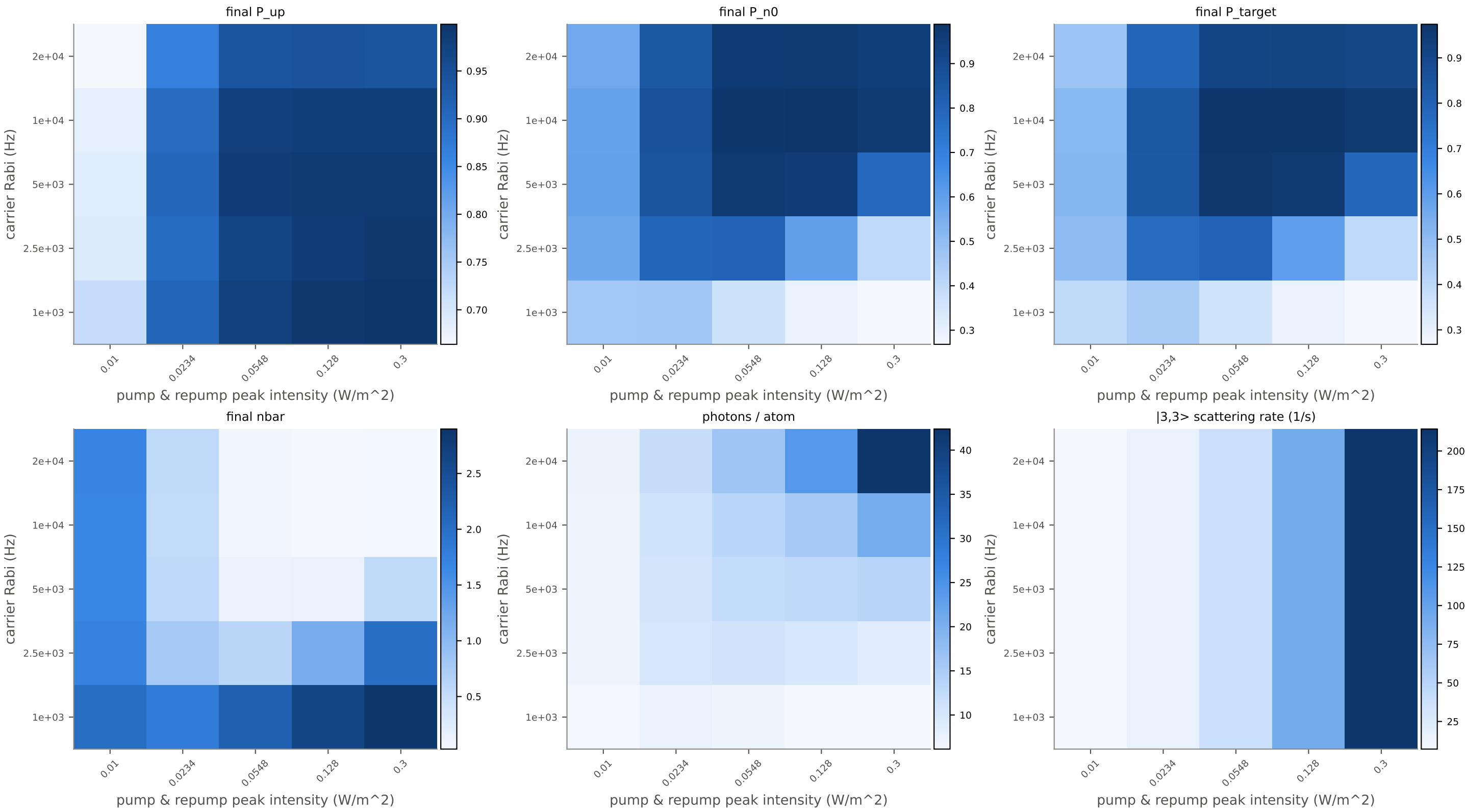
Pump/repump intensity vs Raman carrier Rabi (continuous, 5 ms)
