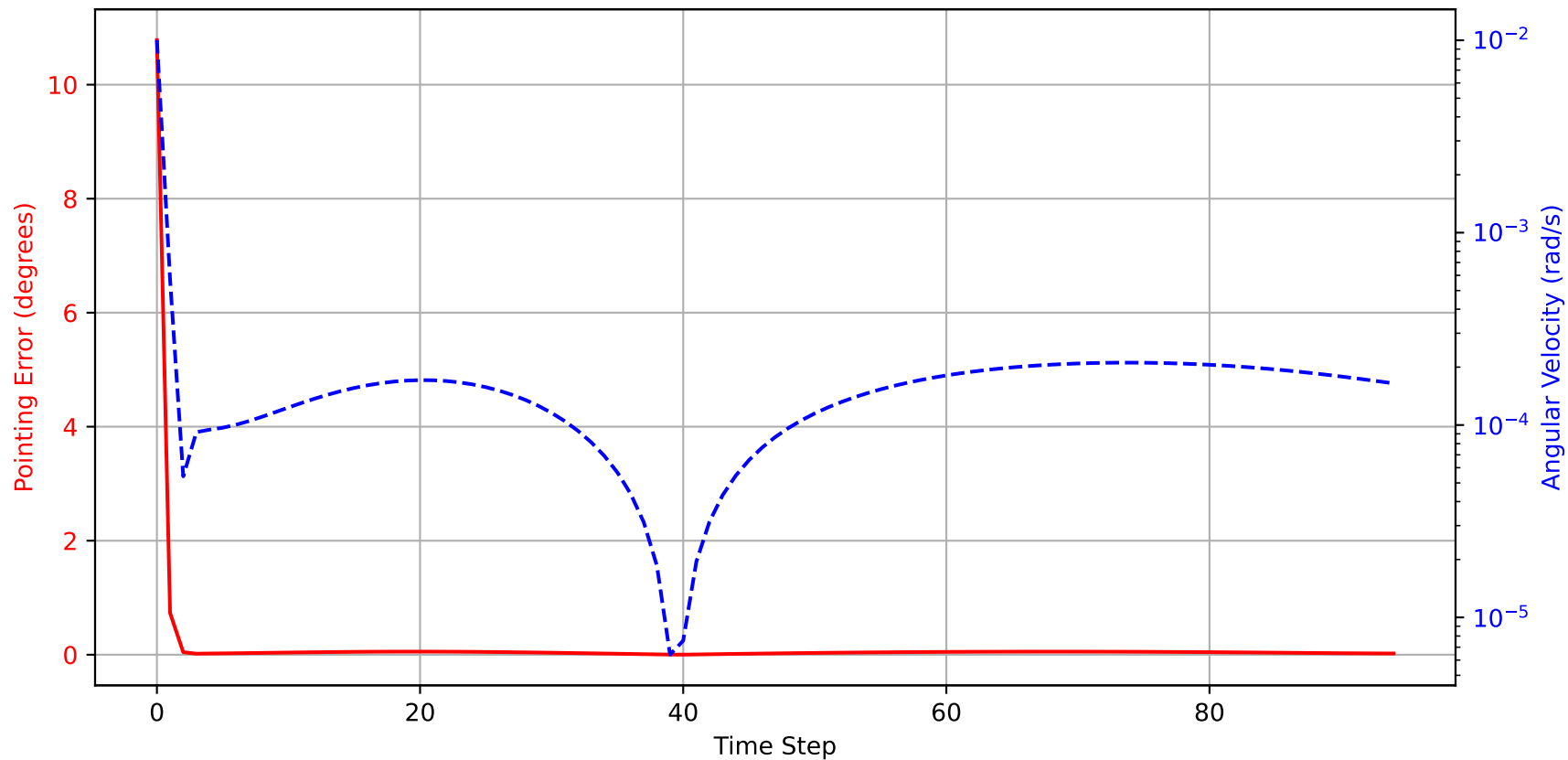
Inspector Satellite Pointing Error and Angular Velocity Over Time
