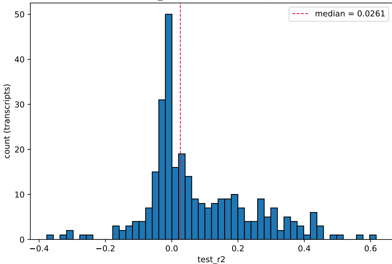
test_r2 across 298 transcripts
