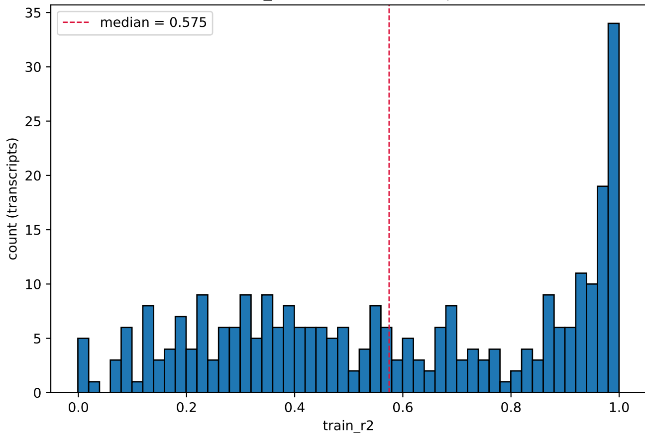
train_r2 across 298 transcripts
