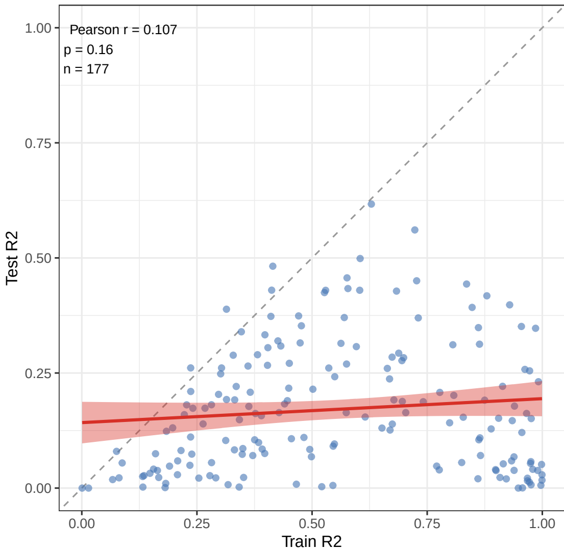
Train vs test R2 per transcript
