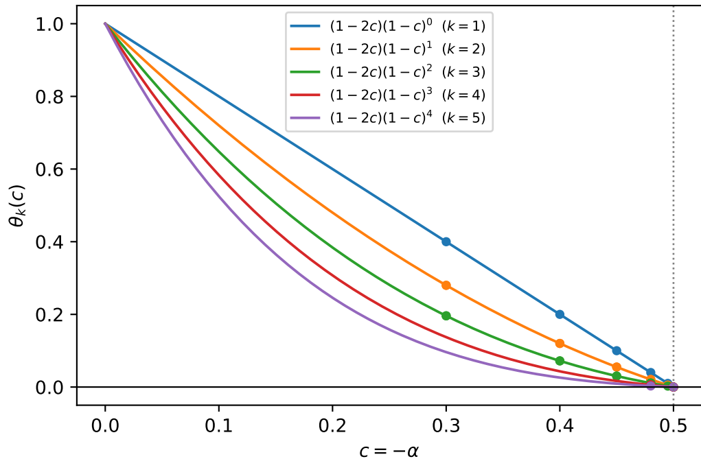
Measured \theta_k vs the padded bound (markers: global search, all d )
