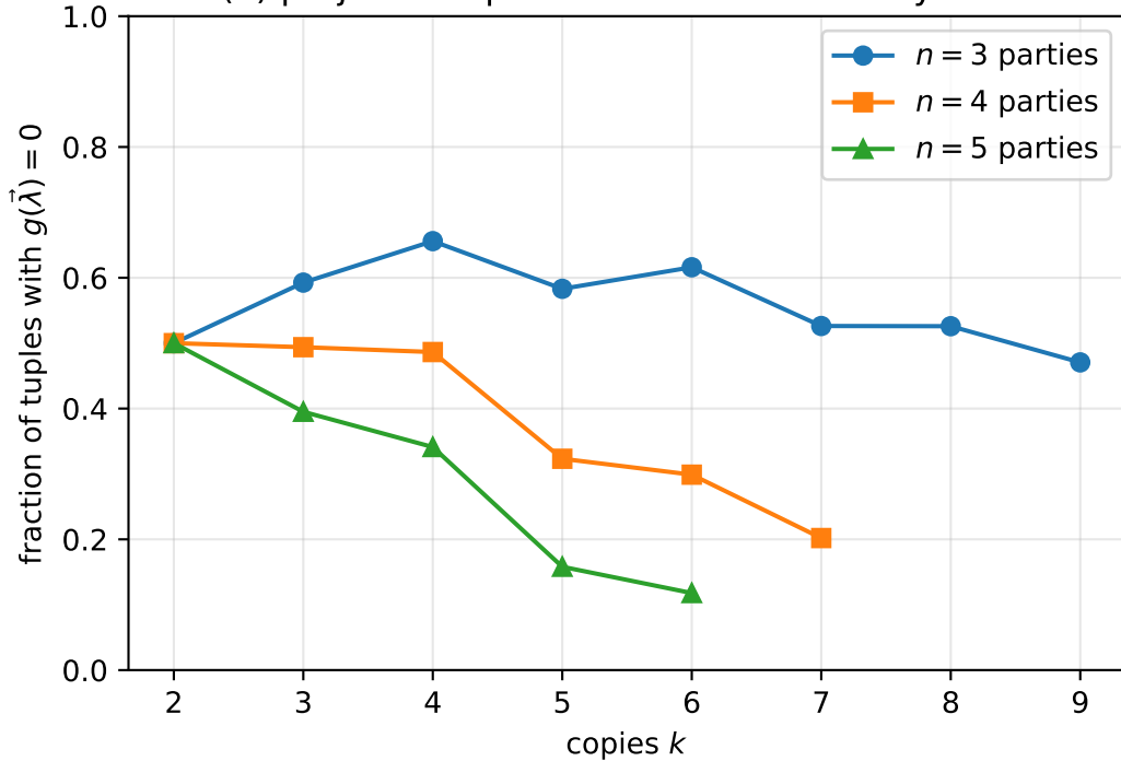
(a) projector tuples that annihilate every state
