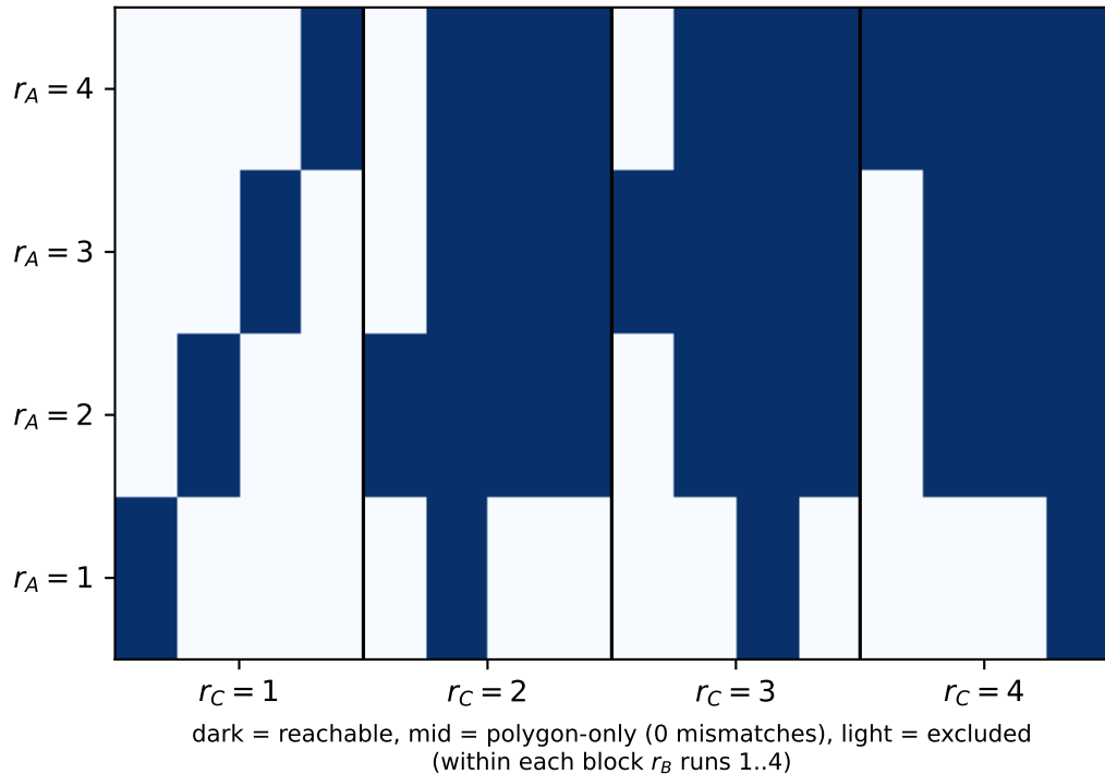
(b) n = 3, k = 7 : reachable rank triples vs polygon
