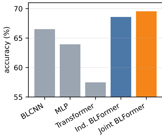
(c) Baselines vs. BLFormer
