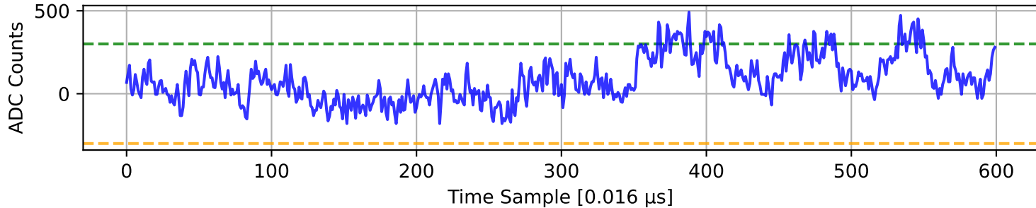
ADC 2 Channel 54
