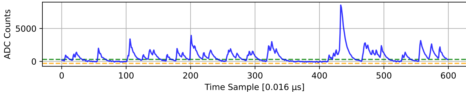
ADC 3 Channel 57
