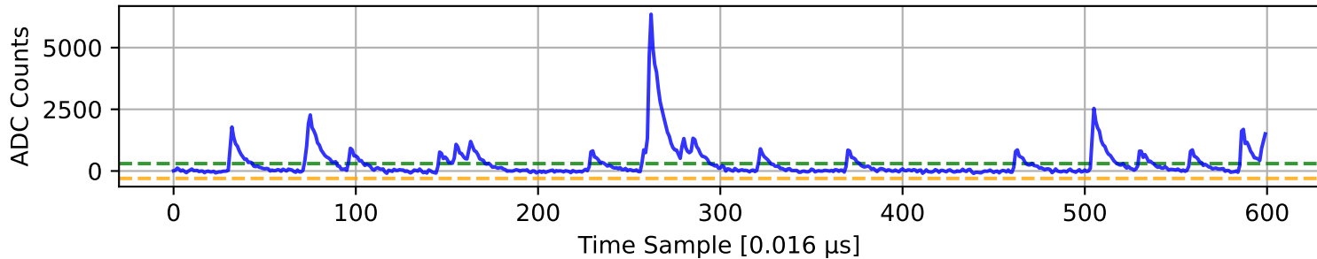
ADC 2 Channel 30
