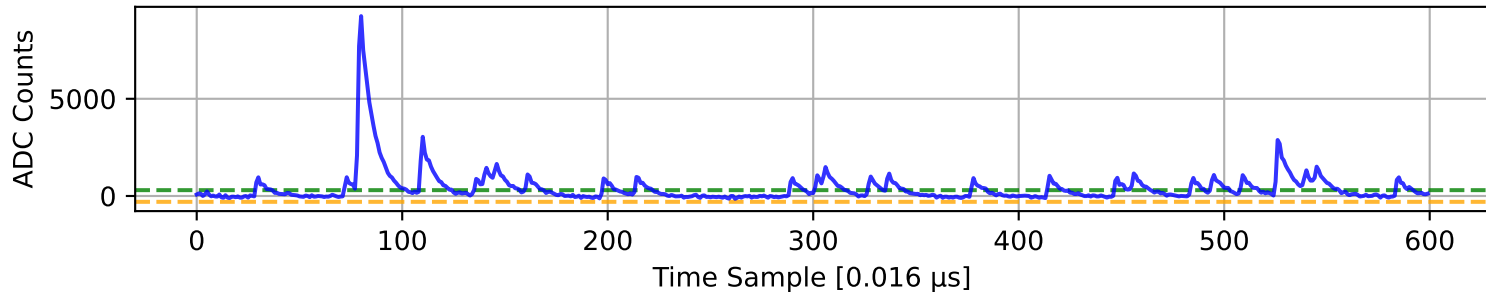
ADC 3 Channel 24
