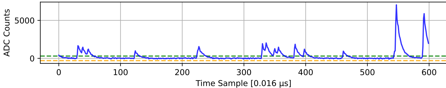
ADC 2 Channel 7
