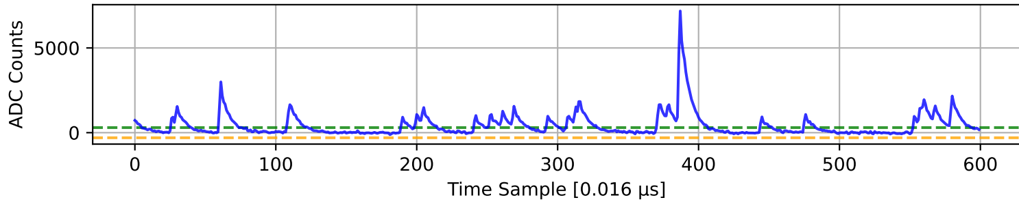
ADC 2 Channel 24
