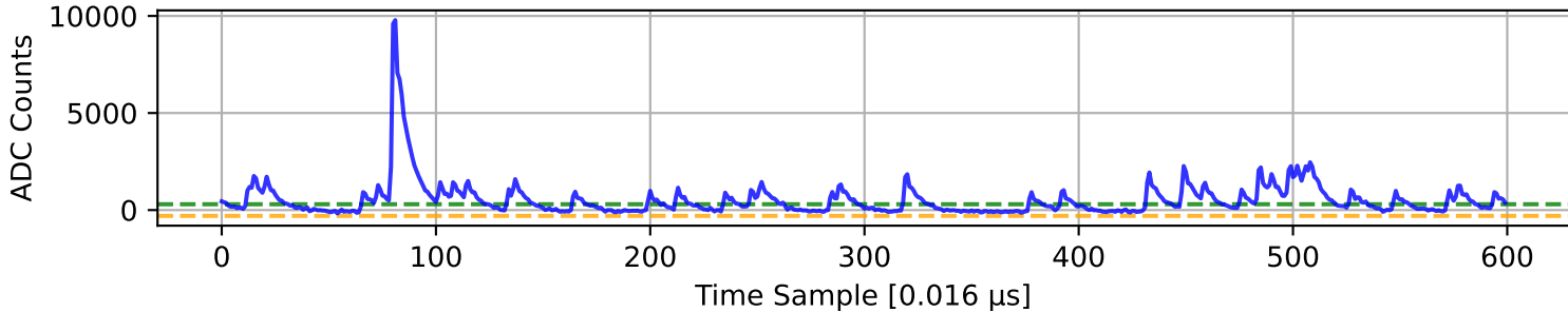
ADC 7 Channel 13
