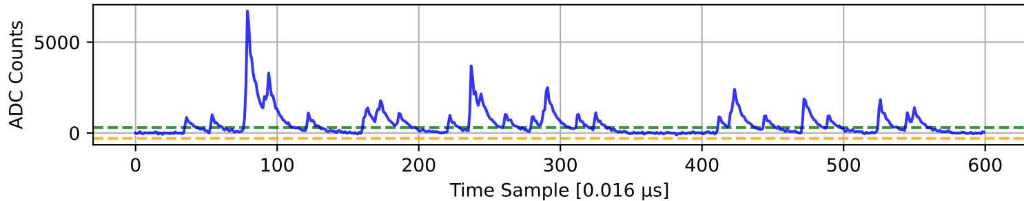
ADC 2 Channel 45
