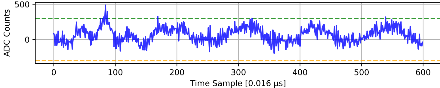
ADC 6 Channel 39
