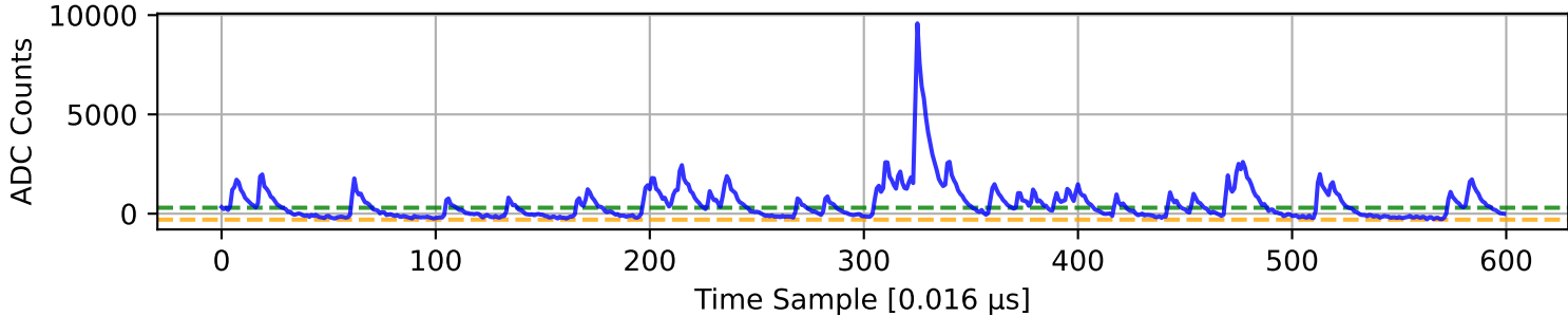
ADC 6 Channel 6
