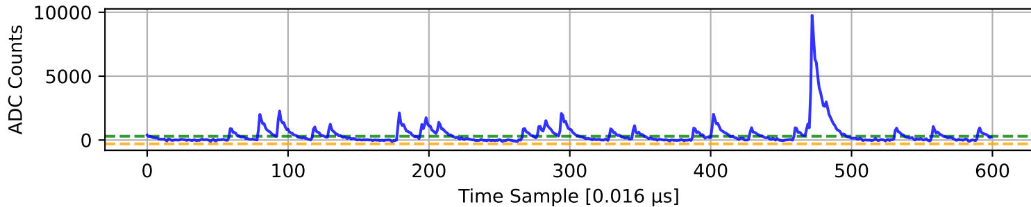
ADC 2 Channel 44
