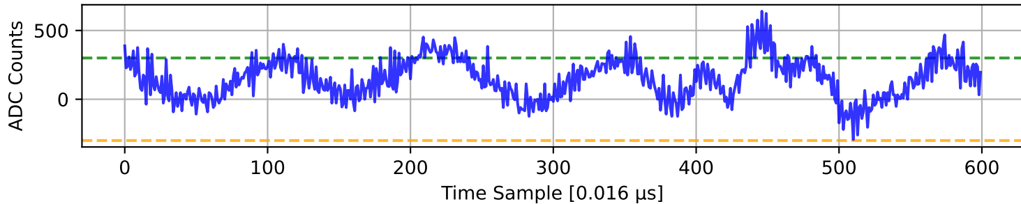
ADC 6 Channel 37
