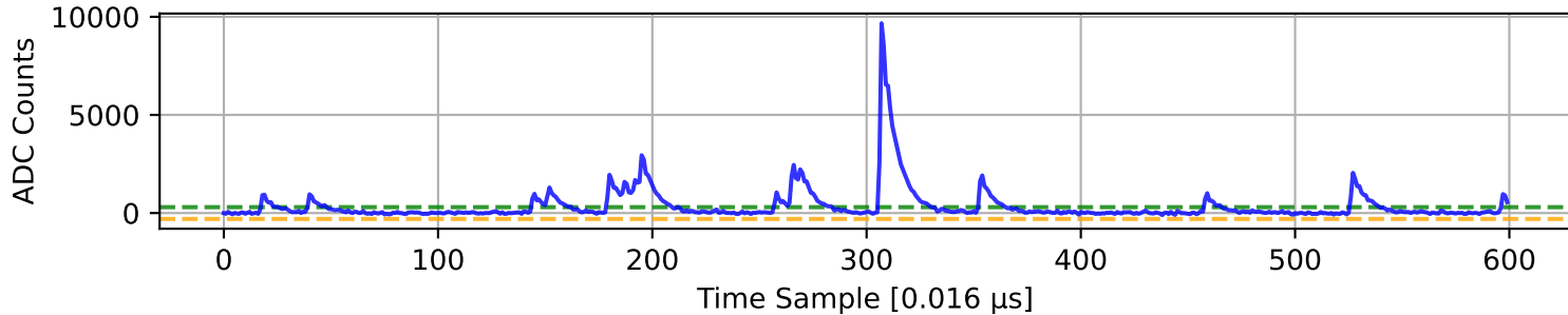
ADC 7 Channel 43
