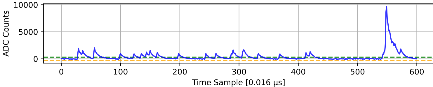
ADC 5 Channel 62
