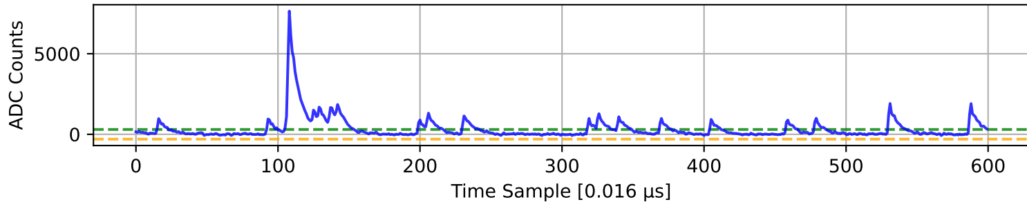
ADC 2 Channel 25
