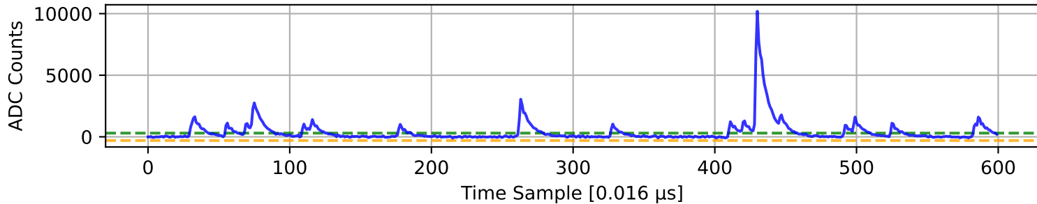
ADC 3 Channel 6
