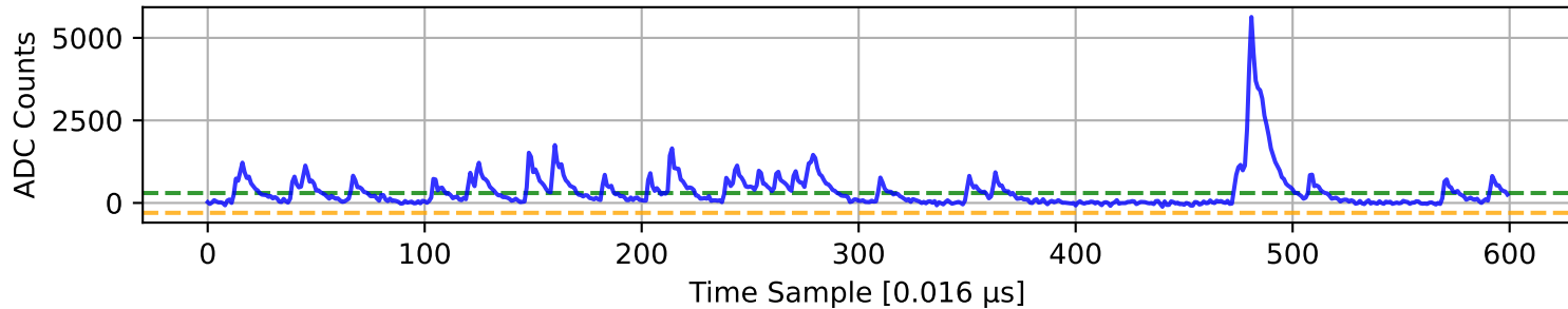
ADC 6 Channel 57
