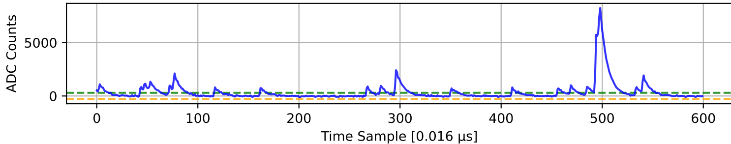
ADC 4 Channel 12
