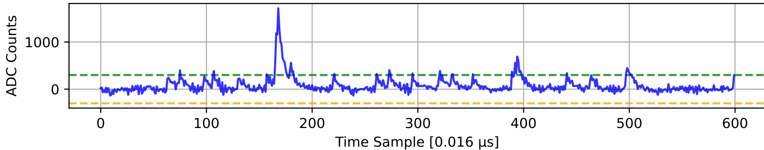
ADC 0 Channel 12
