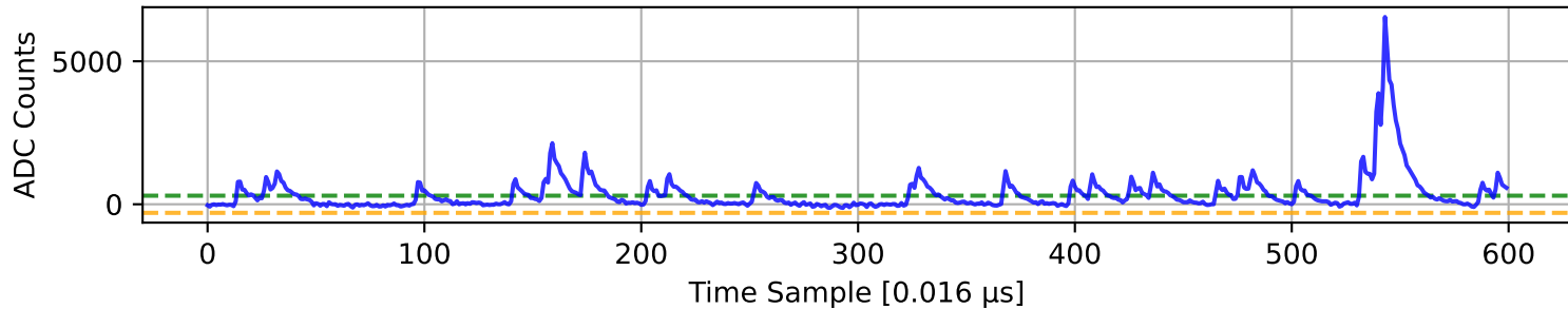
ADC 5 Channel 37
