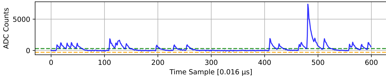
ADC 5 Channel 12
