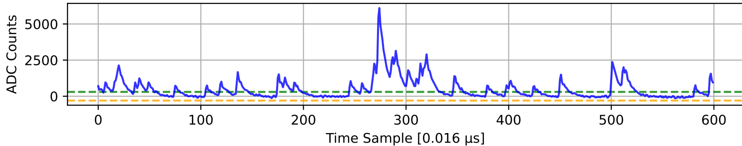
ADC 6 Channel 54
