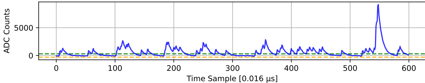
ADC 6 Channel 11
