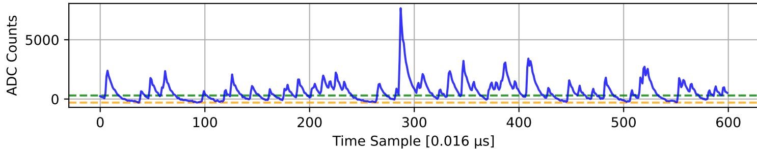
ADC 7 Channel 57
