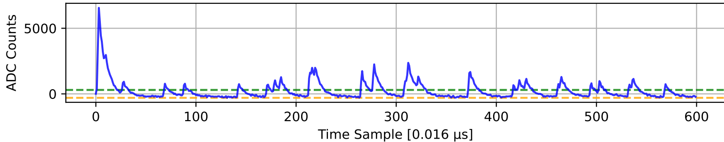
ADC 2 Channel 21
