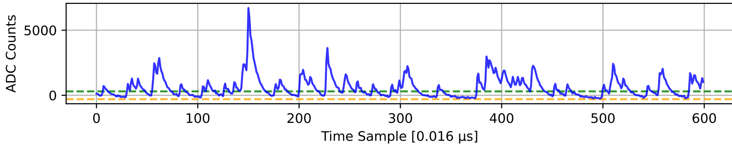
ADC 3 Channel 57
