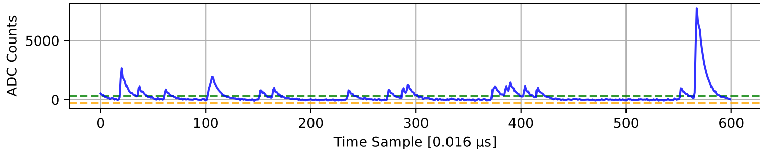
ADC 4 Channel 15
