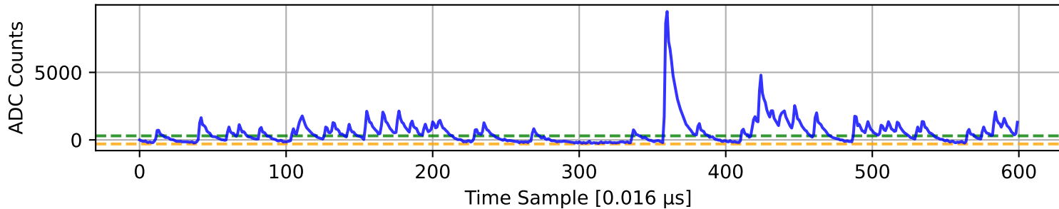
ADC 3 Channel 53
