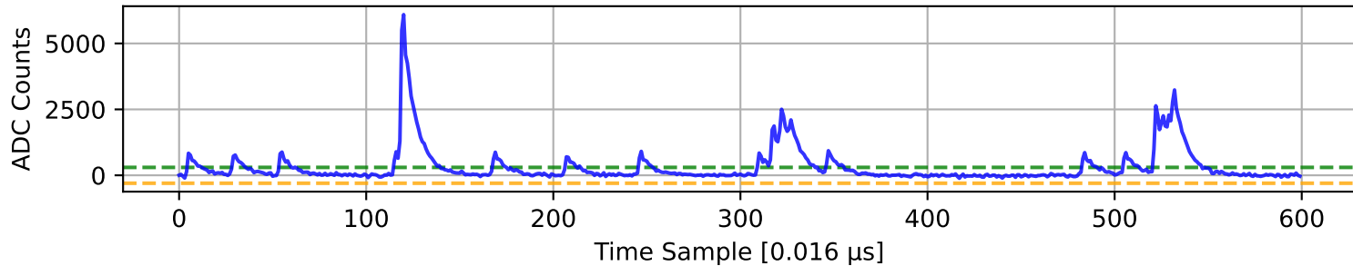
ADC 4 Channel 11
