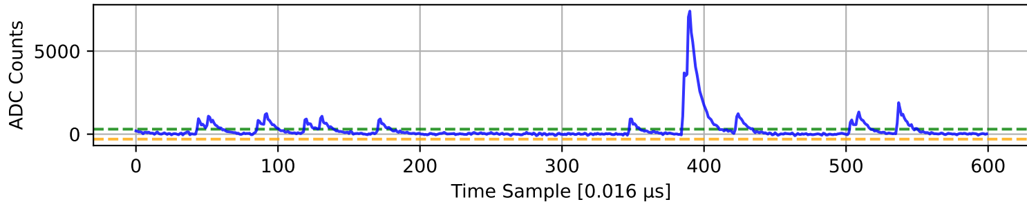
ADC 2 Channel 28
