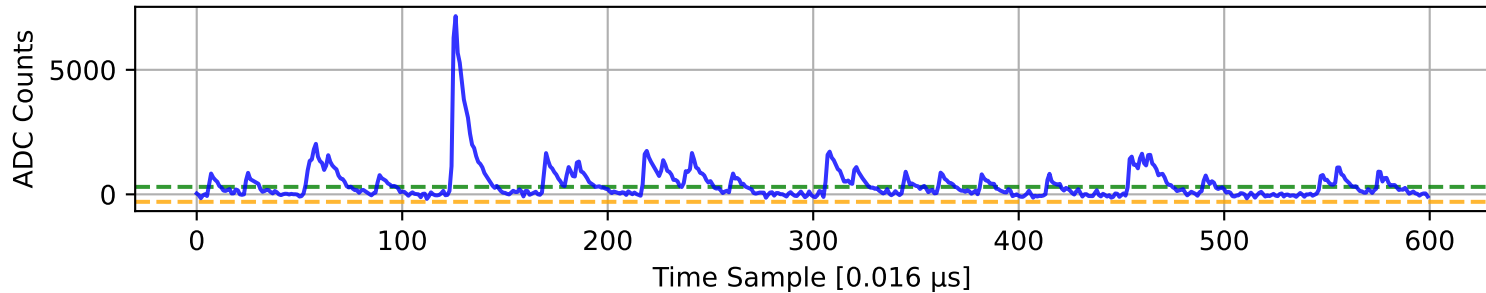
ADC 4 Channel 21
