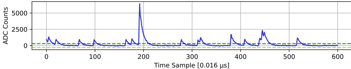
ADC 4 Channel 45
