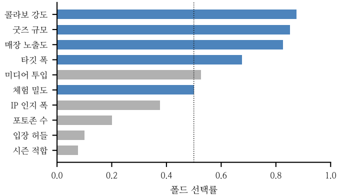
ridge
