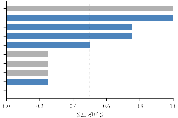
gbdt
