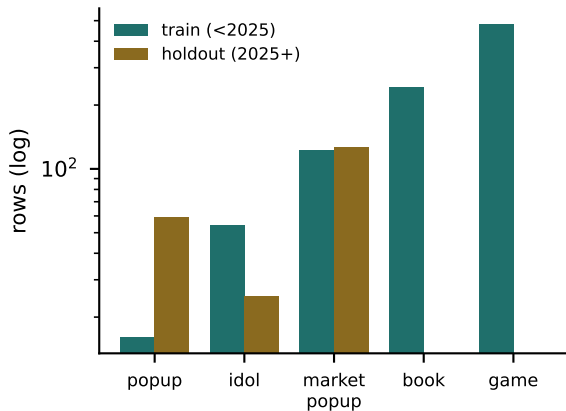
(a) popup: 16 train, 59 holdout holdout is 3.7x train
