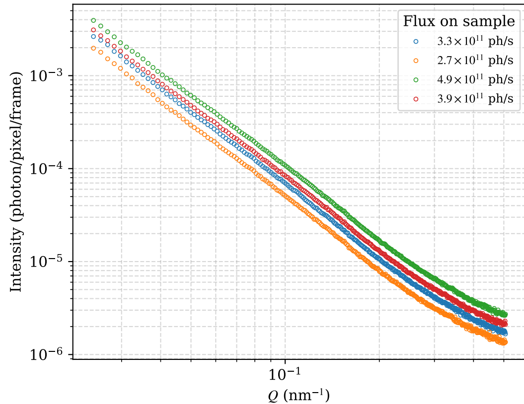
SAXS
