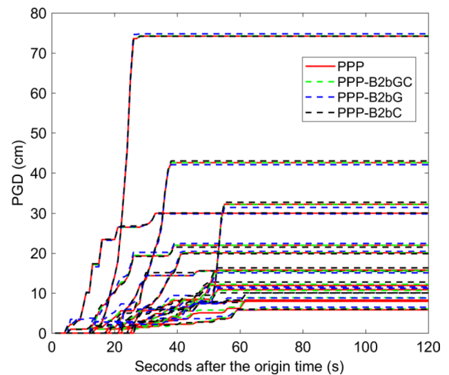
Fig. 5 PGDs extracted in real time from the coseismic displacements of the PPP, PPP-B2bG, PPP-B2bC and PPP-B2bGC for all GNSS stations
