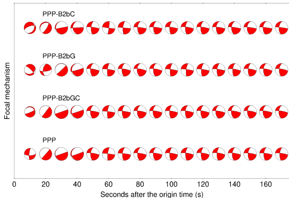
Fig. 8 Focal mechanisms derived from the CMT results inverted with the different static coseismic offsets. For clarity, the focal mechanisms are displayed with an interval of 10 s
