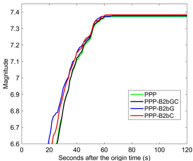
Fig. 6 Time series of the warning magnitudes determined with different GNSS PGDs
