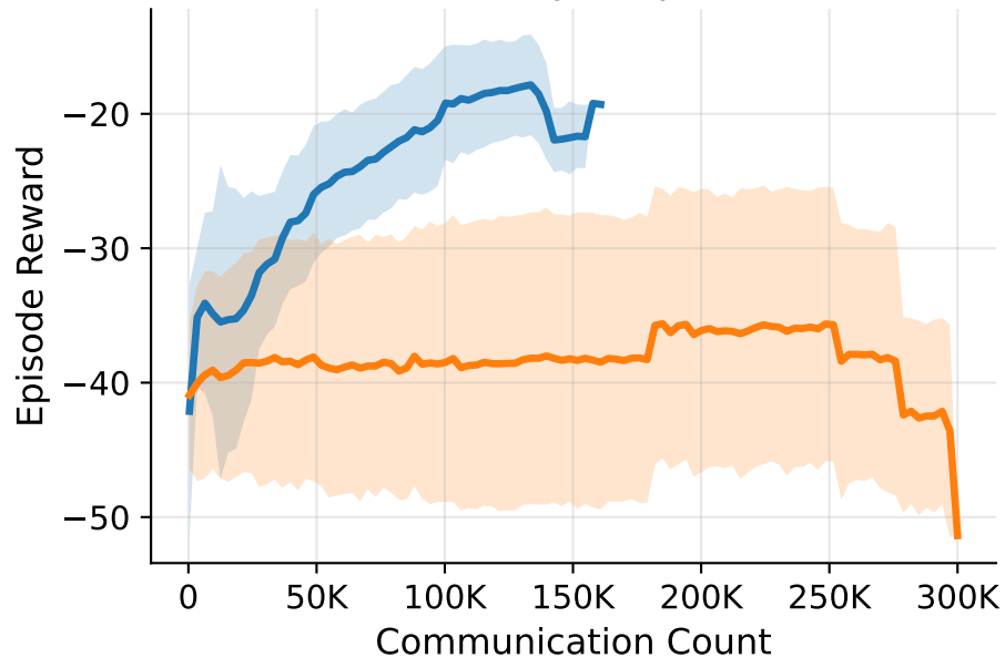
MPE Simple Spread
