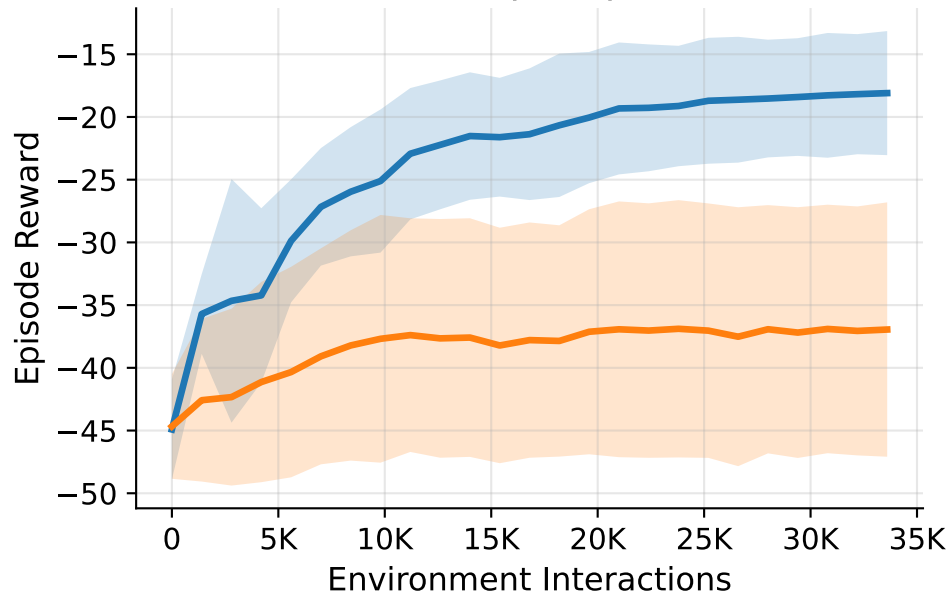
MPE Simple Spread
