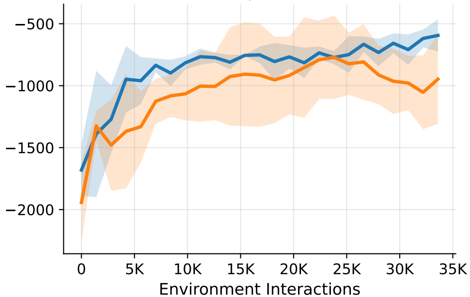
MPE Simple Facmac
