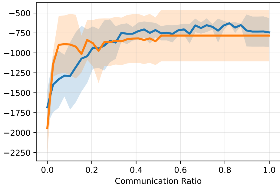
MPE Simple FACMAC
