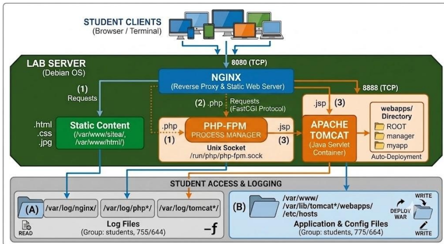
Figure 1: Lab1 setup
