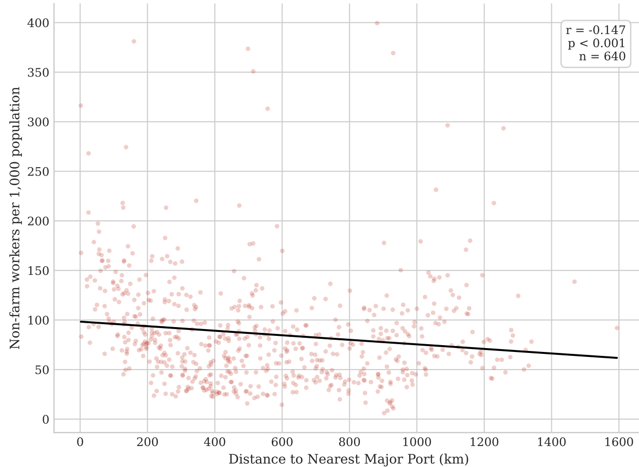
(a) Port Proximity
