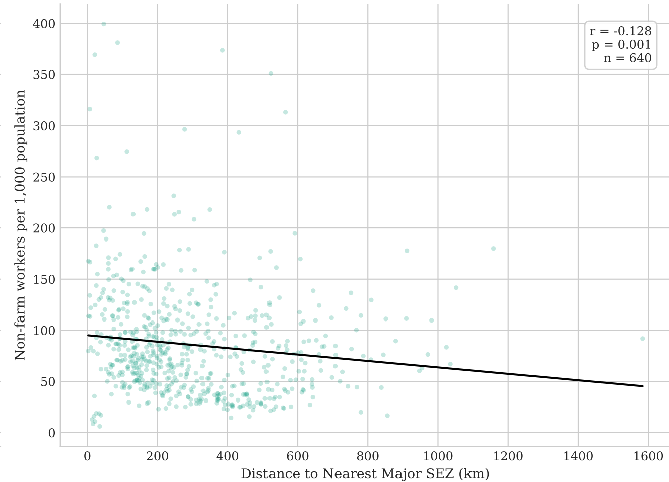
(b) SEZ Proximity
