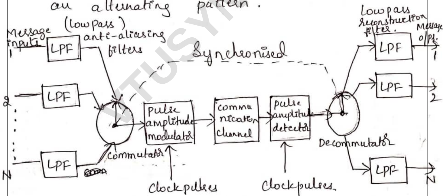
fig: Block diagram of TDM system.
