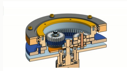
Actuator section render
