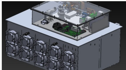
Accumulator attic CAD
