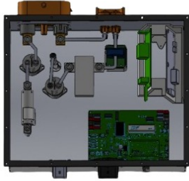
Top-down attic CAD view used to check electronics layout and access.
