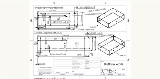
Bottom wall drawing with datums, critical dimensions, and positional tolerance callouts.
