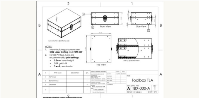
Assembly drawing defining lid, latch, hinge, body, and insert interfaces.
