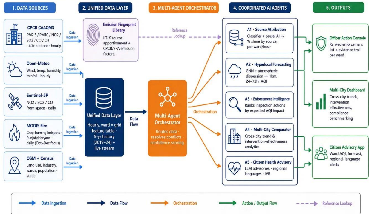
Figure 1. PRAANA system architecture — data sources, unified data layer, multi-agent orchestrator, and output surfaces.
