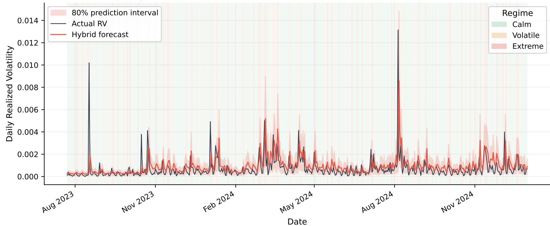
BTC: Hybrid LSTM + IT2FIS Forecast vs Actual Realized Volatility (Test Period)
