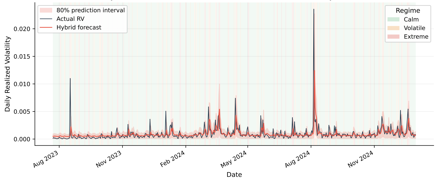
ETH: Hybrid LSTM + IT2FIS Forecast vs Actual Realized Volatility (Test Period)
