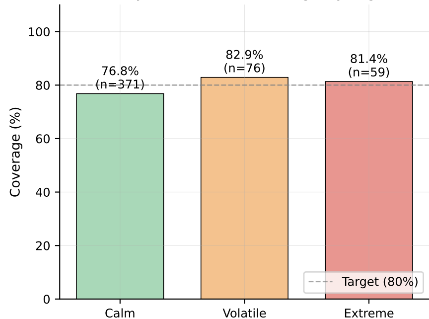
BTC: Hybrid interval coverage by regime
