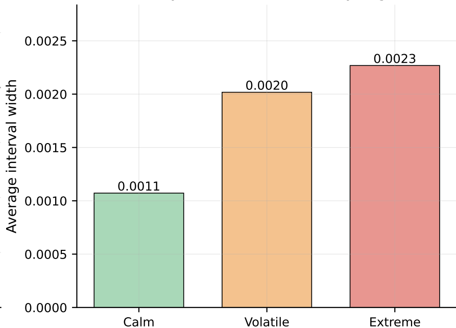
BTC: Hybrid interval width by regime
