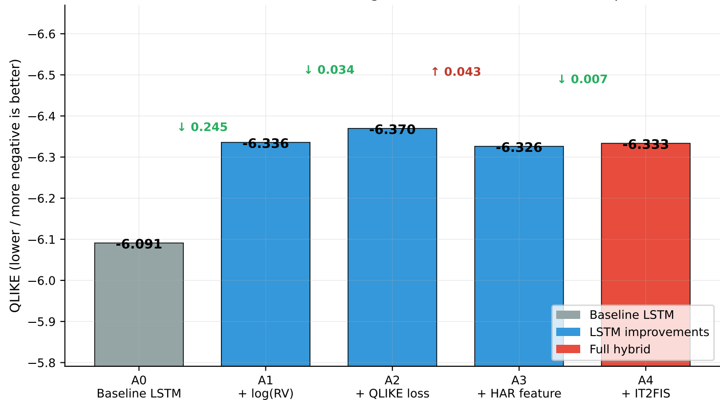
BTC: Cumulative Ablation — Marginal Contribution of Each Component
