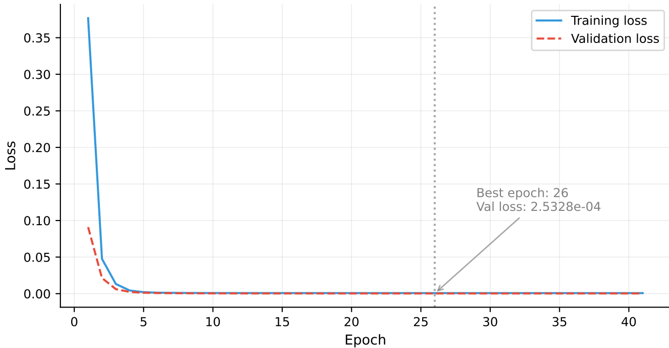
ETH: LSTM v2 Training Curves (log target + QLIKE + HAR)
