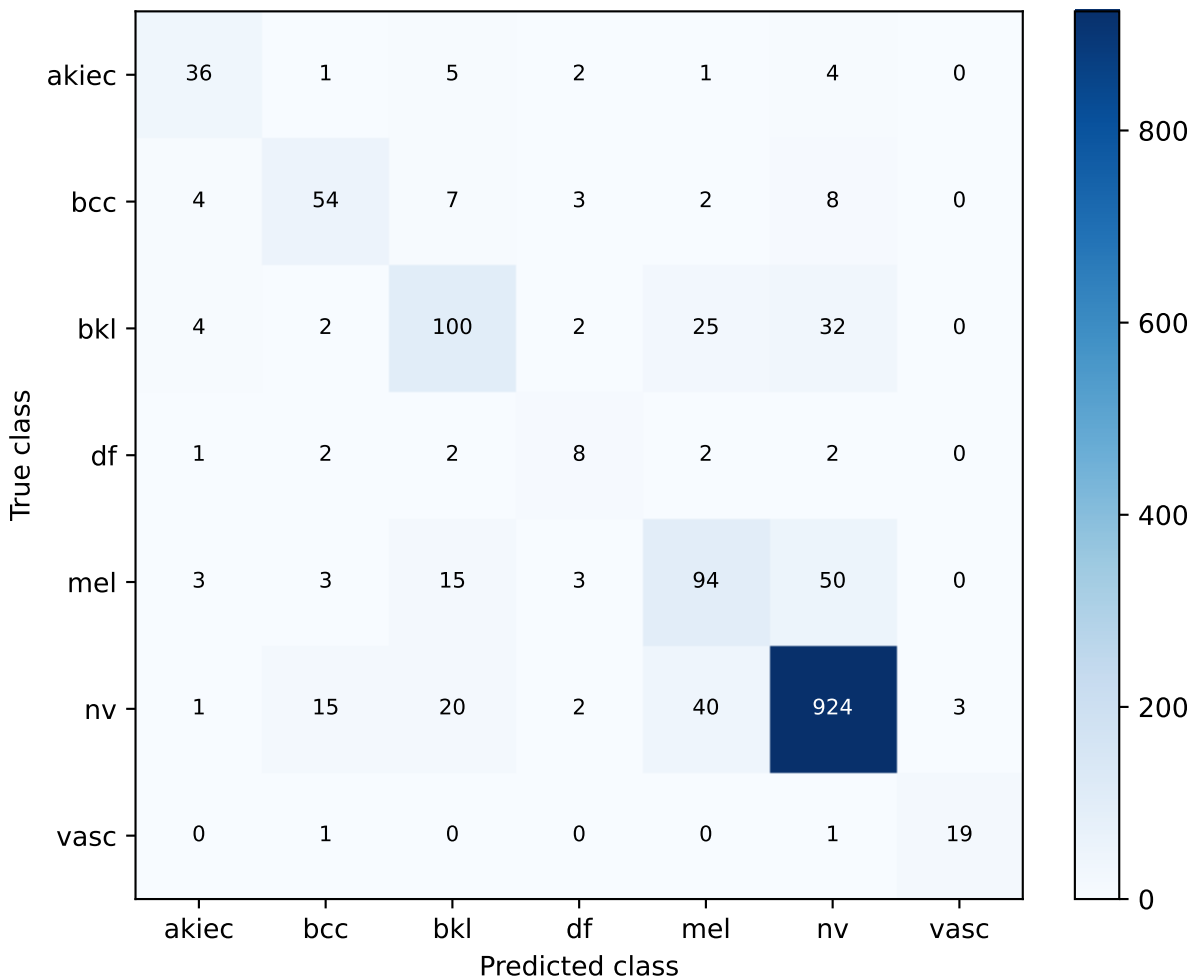
efficientnet_b0 | final locked test Confusion matrix
